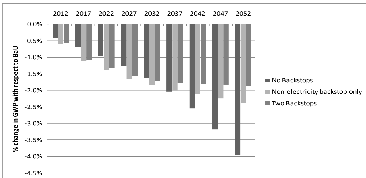
Figure 6. Costs (% GWP difference with BAU) of a 450 ppm CO 2 (550 ppm CO 2 eq) concentration stabilisation policy under alternative assumptions regarding investment possibilities in advanced technologies.
